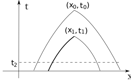
FIGURE 2. Proof of Theorems 2.1 and 2.3.
