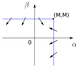
FIGURE 1. \max\{\alpha, \beta\} < M is an invariant domain. Note: \alpha (or \beta ) might increase along characteristic.
