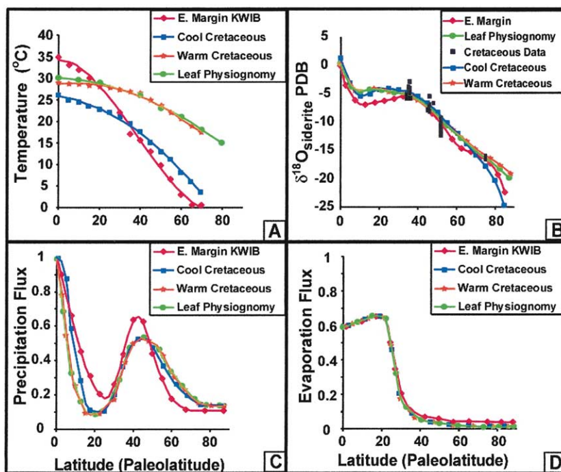
Fig. 8. (A) The four gradients illustrated represent the thermal gradients (with best-fit polynomial curves) that were embedded in the mass balance model to test temperature sensitivity. The warm and cool Cretaceous curves were obtained from Barron (1983) , the E. Margin KWIB curve is from Poulsen et al. (1999) , and the Leaf Physiognomy curve is from Wolfe and Upchurch (1987) (in Spicer and Corfield, 1992 ). (B) With each temperature gradient, it was possible to reproduce a latitudinal gradient that fits the Albian siderite \delta^{18}\text{O} values. (C) Each curve represents the input precipitation flux profile that generates the siderite \delta^{18}\text{O} gradient illustrated in B. (D) The input evaporation flux curves for each of the four tests are illustrated; however, only very minor changes were required in one of the tests (E. Margin KWIB temperature gradient).
