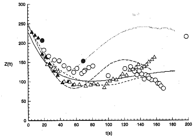
Fig. 11 Comparison between measured and simulated vertical vortex (center) position histories for B 767 tower flyby tests (see Fig. 5 for legend).
