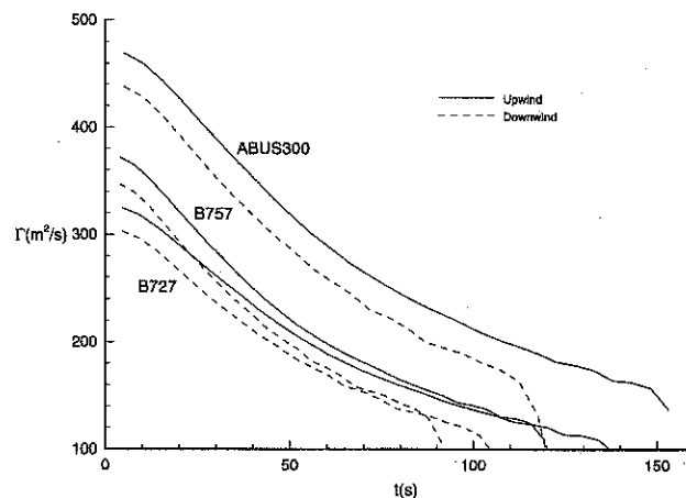
Fig. 13 Representations of circulation decay histories for three aircraft types subjected to surface weather conditions represented by run 9.
