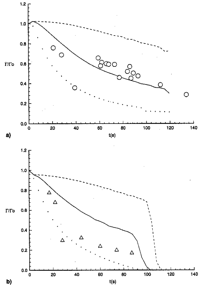
Fig. 3 Influence of equivalent Reynolds number on computed decay rate of wake vortices when subjected to run 9 weather conditions represented. \circ , measured upwind vortex circulation; \Delta , measured downwind circulation; —, R = 800 ; ---, R = 3000 ; ..... , R = 300 . Comparison of a) upwind and b) downwind vortices.
