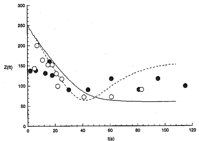
Fig. 12 Comparison between measured and simulated vertical vortex (center) position histories for B 727 tower flyby test designated as run no. 22 (see Fig. 6 for legend).
