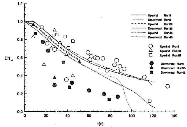
Fig. 4 Comparison between measured and simulated circulation decay histories for three B 757 tower flyby tests. See Table 1 and Figs. 1 and 2 for more details.
