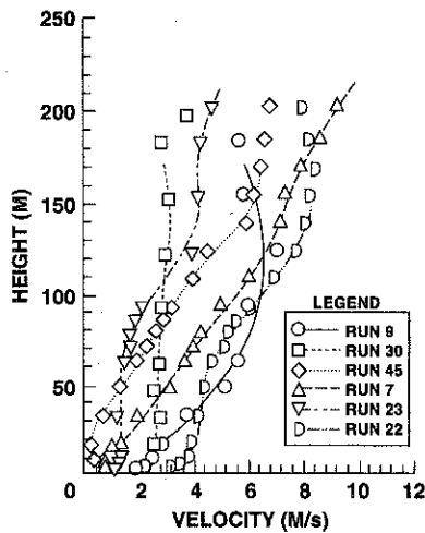
Fig. 1 Measured surface wind velocity profiles for the six Idaho Falls flight tests defined in Table 1. The corresponding curves represent the polynomial data fits used in the numerical simulations.
