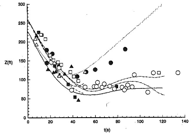
Fig. 10 Comparison between measured and simulated vertical vortex (center) position histories for B 757 tower flyby tests (see Fig. 4 for legend).
