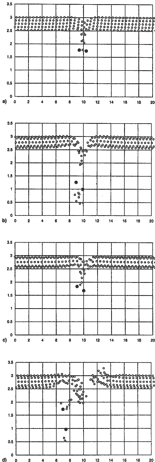
Fig. 3 Vortex position histories with shear layer above. The symbols have the same meaning as those in Fig. 1a: a) 2% shear at t = 1.6 , b) 2% shear at t = 5.6 , c) 10% shear at t = 1.6 , and d) 10% shear at t = 5.6 .
