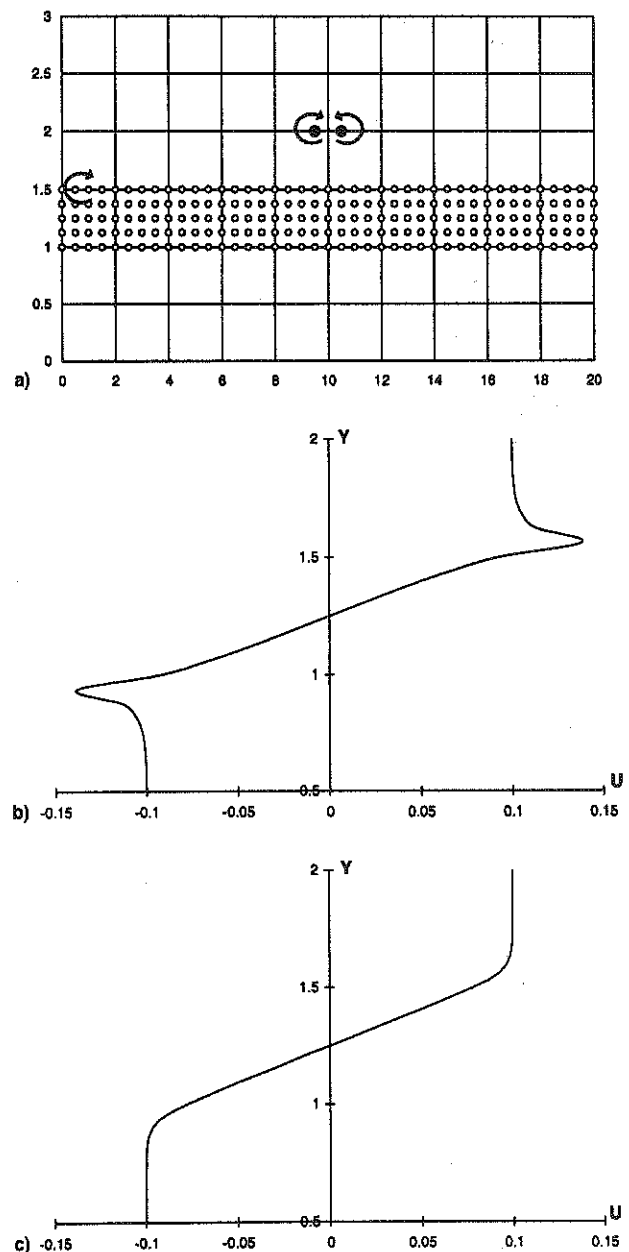
Fig. 1 Initial flowfield: a) Vortex positions. \bullet = the two vortices in the vortex wake, and \circ = the vortices in the shear layer. b) Velocity in x direction, u , vs height, y , at x locations aligning on the shear vortices. c) Velocity in x direction, u , vs height, y , at x locations between the shear vortices.
